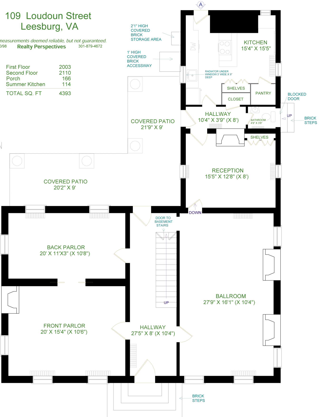
FIRST FLOOR
